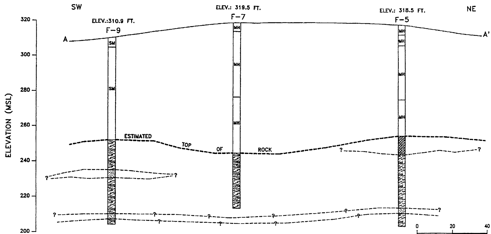
Figure 2-12 ISFSI SUBSURFACE CROSS SECTION
